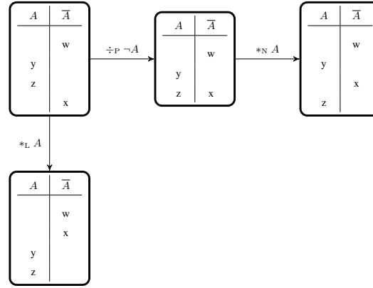
Fig. 7: Countermodel establishing Proposition 22.
