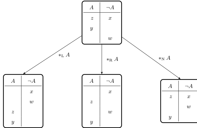
Fig. 1: Revision by A according to the operators *_{\text{L}} , *_{\text{R}} and *_{\text{N}} . The boxes represent states and associated TPOs. The lower case letters, which represent worlds, are arranged in such a way that the lower the letter, the lower the corresponding world in the relevant ordering. The columns group worlds according to the sentences that they validate. So, for example, in the initial ordering, we have w \prec y \prec x \sim z , with y, z \in \llbracket A \rrbracket and x, w \in \llbracket \neg A \rrbracket and then, after lexicographic revision by A , y \prec z \prec w \prec x .
