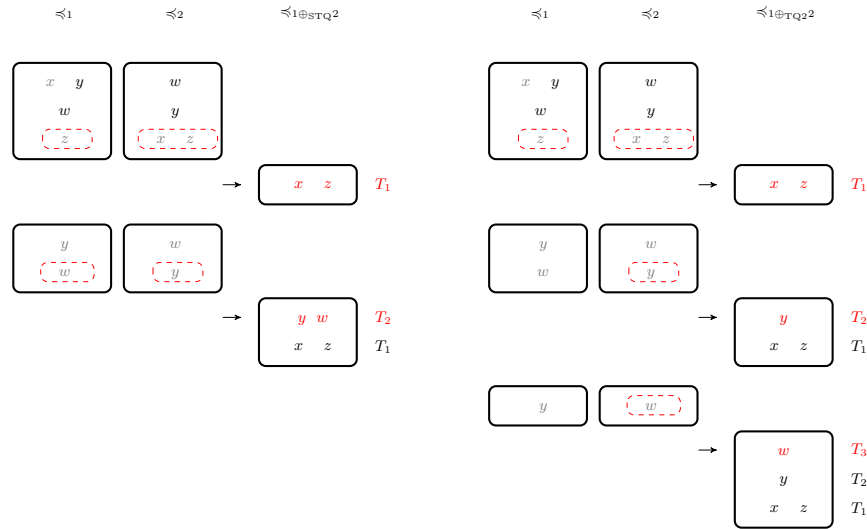
Fig. 2: Illustration of the construction of \preccurlyeq_{1 \oplus 2} in Example 1 (left) and Example 2 (right). This construction in each case is illustrated chronologically from top to bottom.
